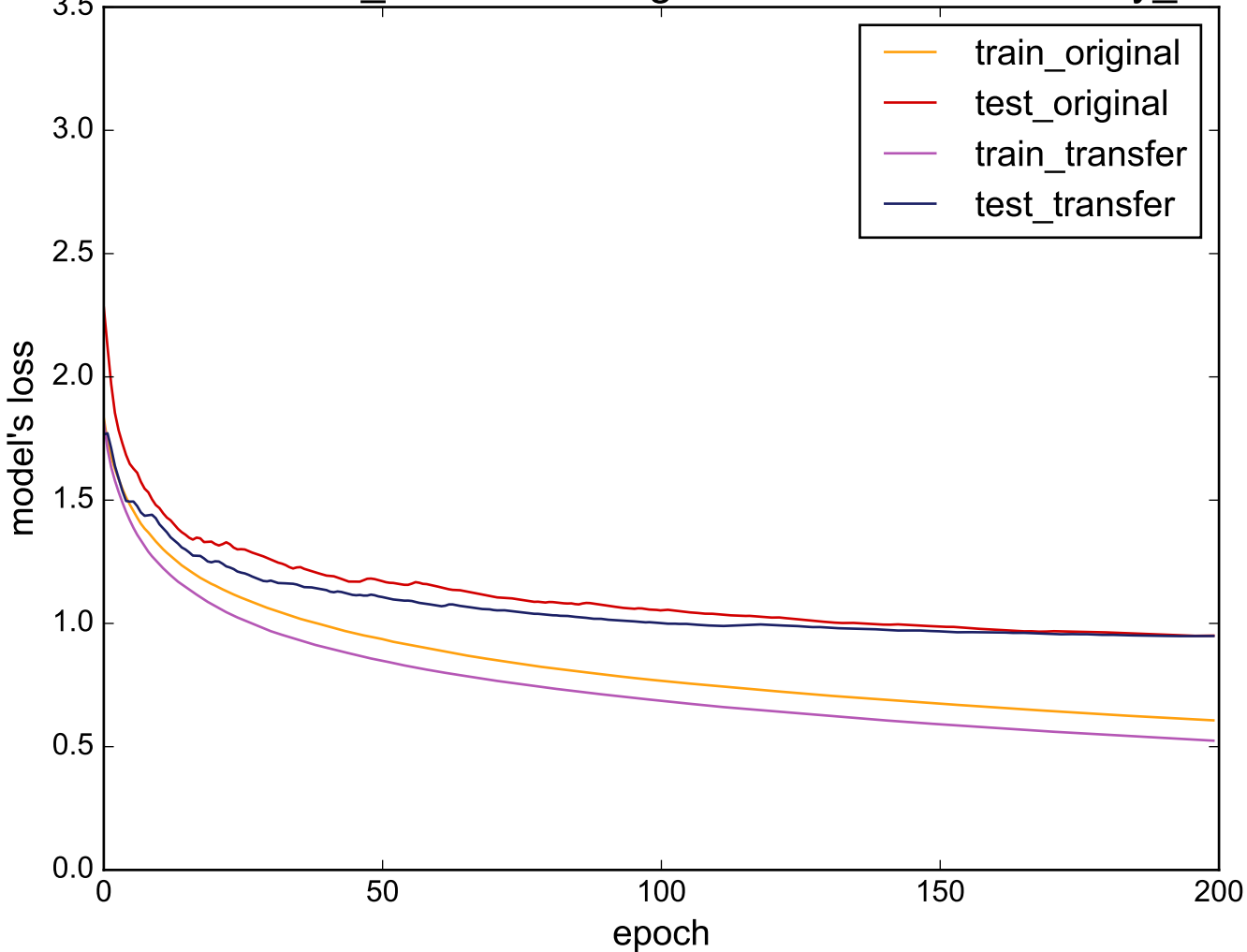
Source: Two_Patterns - Target: uWaveGestureLibrary_X
