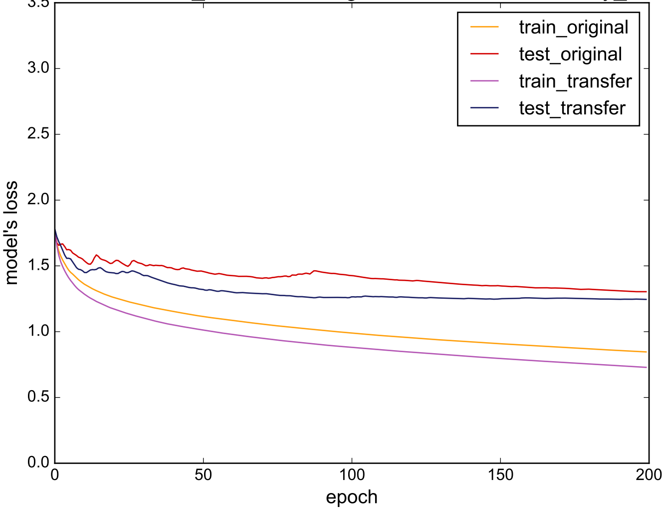
Source: Two_Patterns - Target: uWaveGestureLibrary_Y
