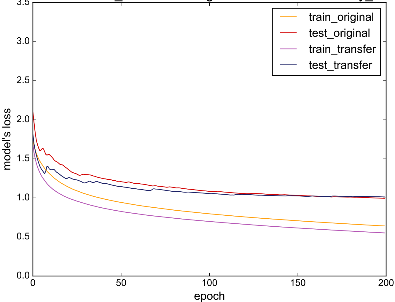
Source: Two_Patterns - Target: uWaveGestureLibrary_Z
