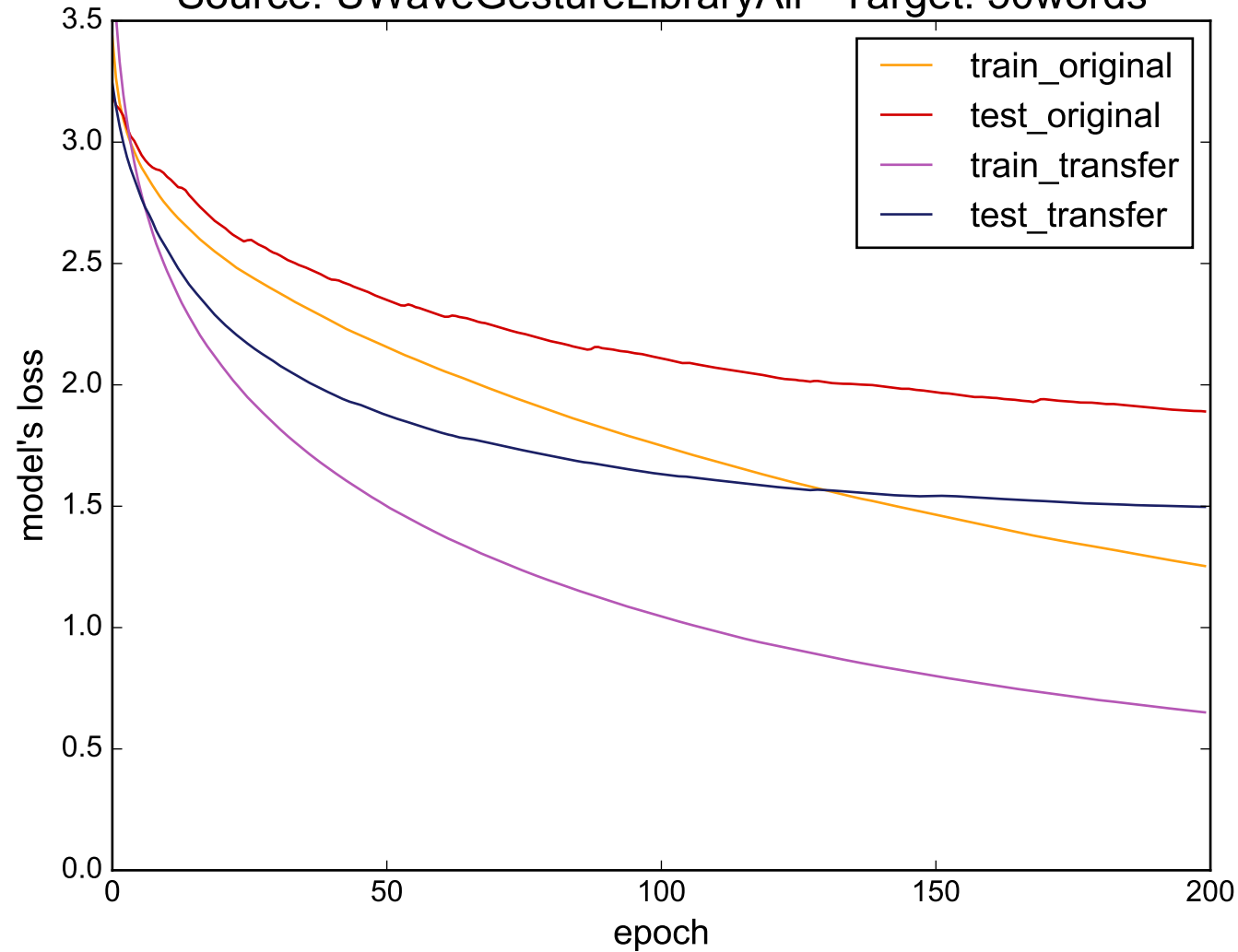
Source: UWaveGestureLibraryAll - Target: 50words
