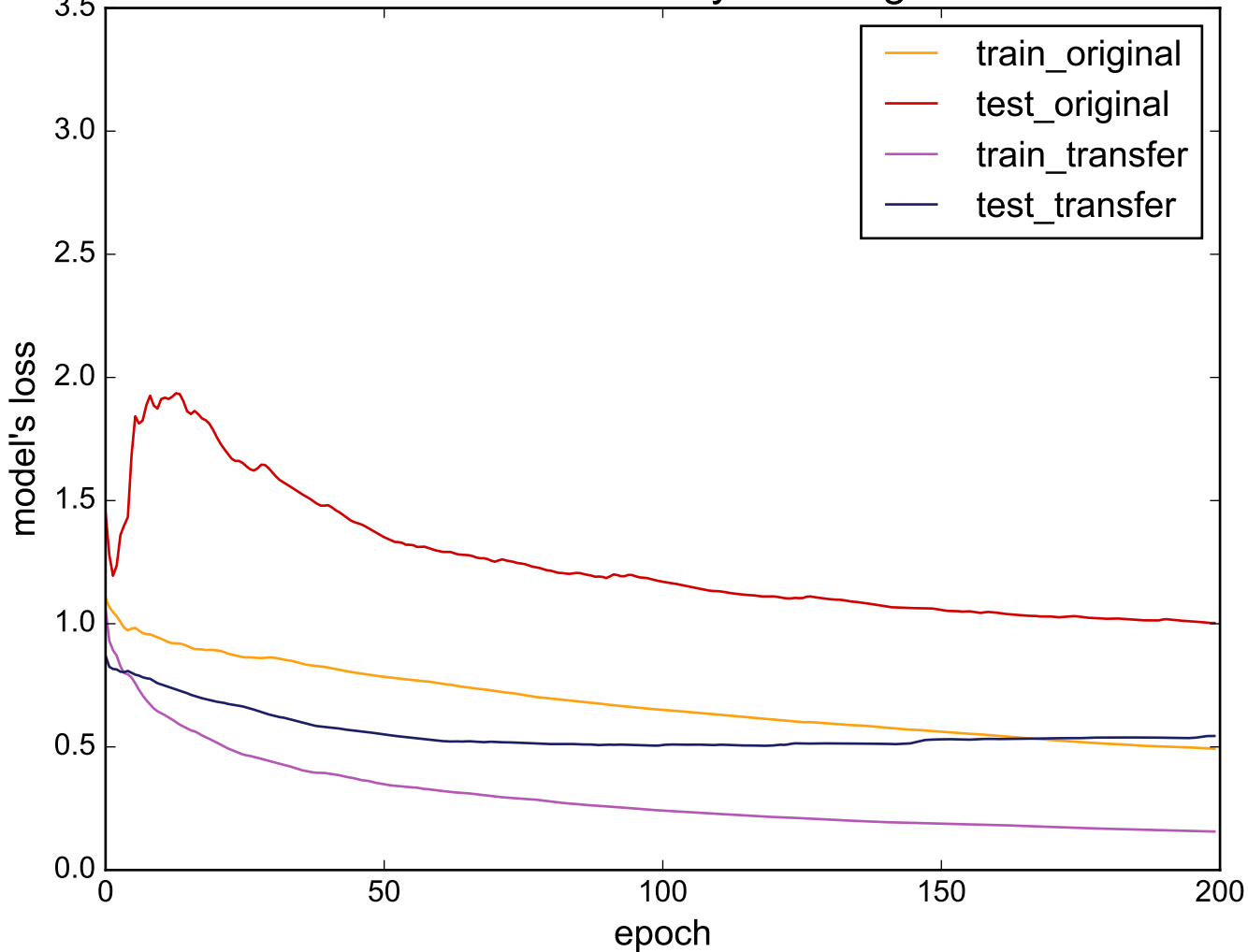
Source: UWaveGestureLibraryAll - Target: ArrowHead
