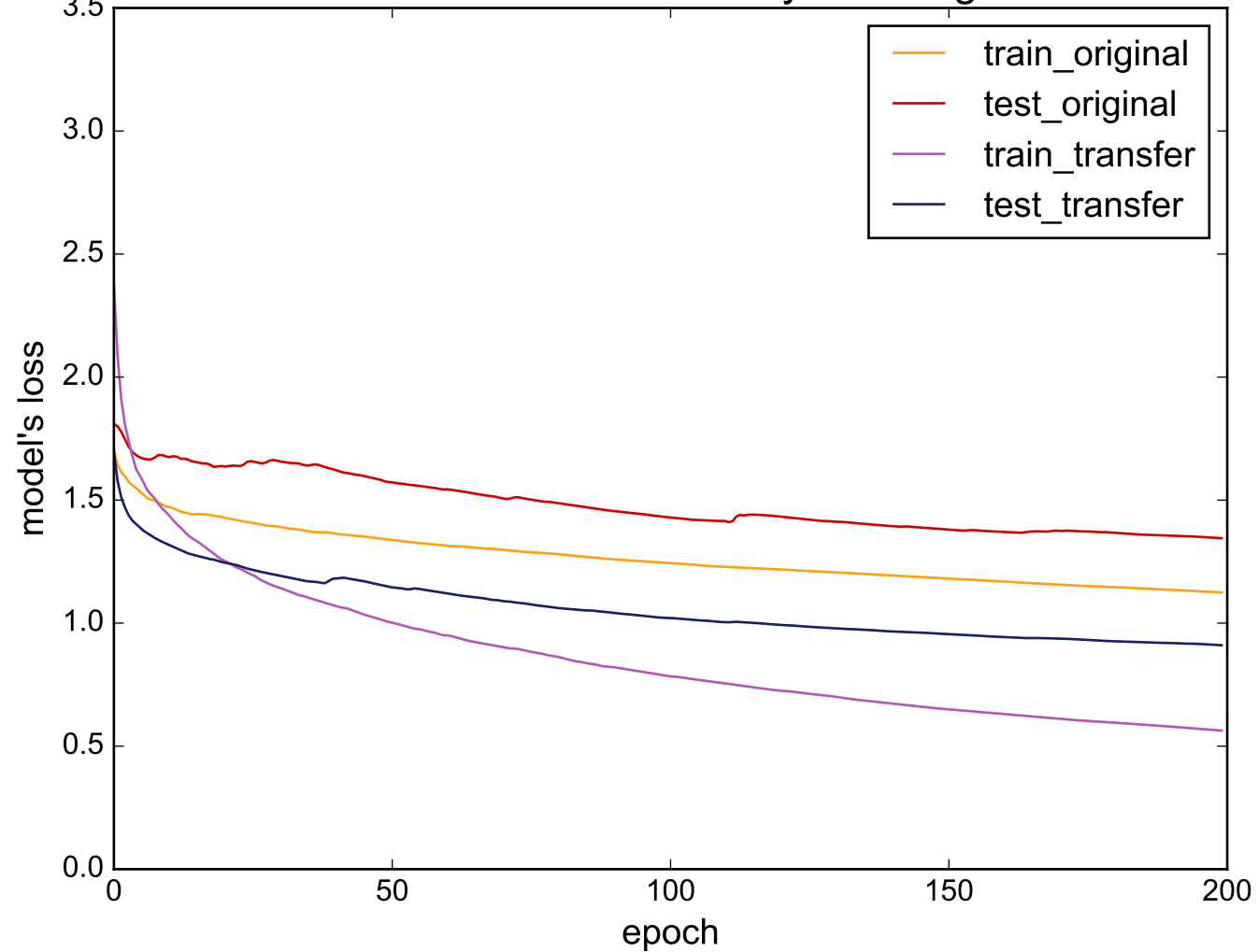
Source: UWaveGestureLibraryAll - Target: Beef
