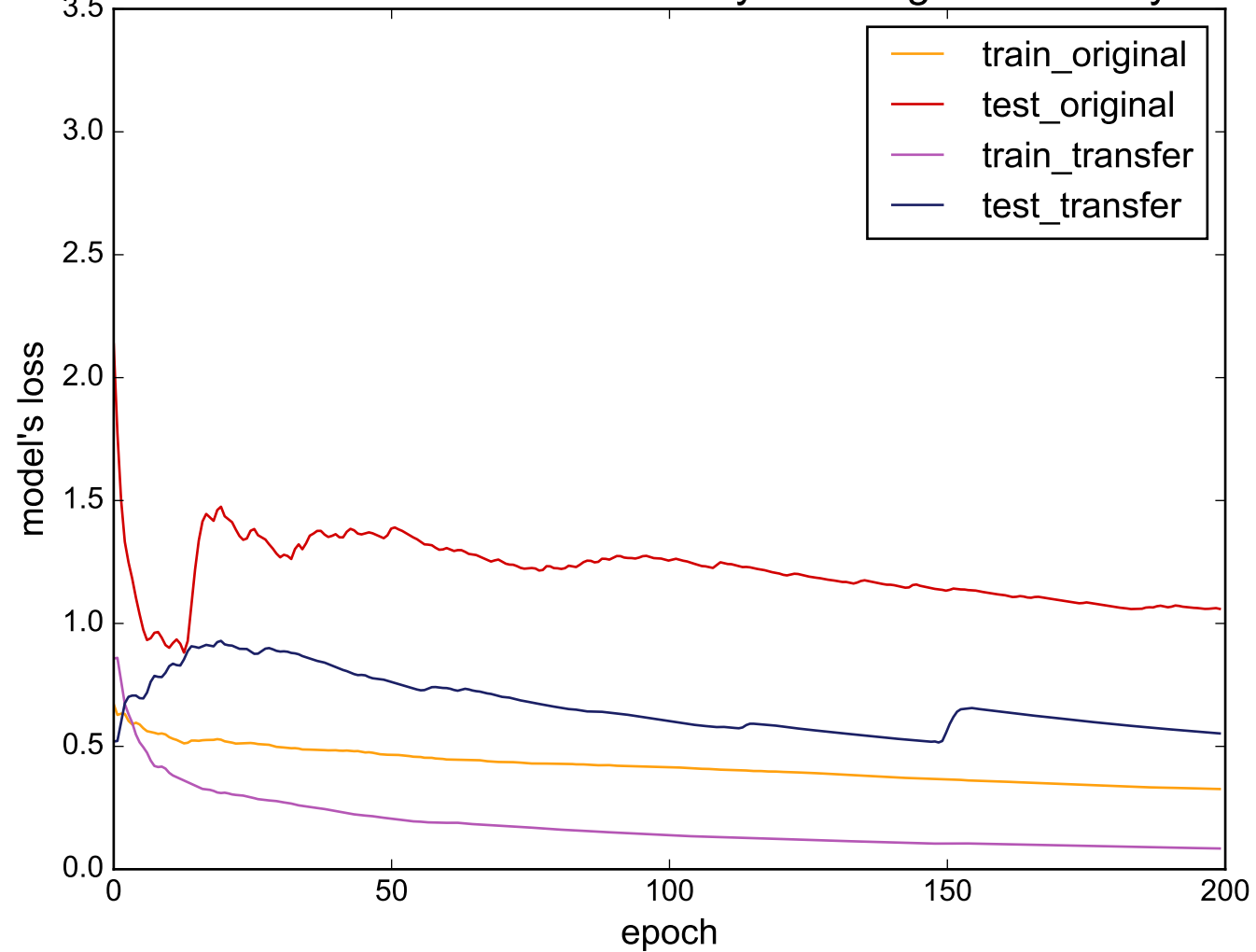
Source: UWaveGestureLibraryAll - Target: BeetleFly
