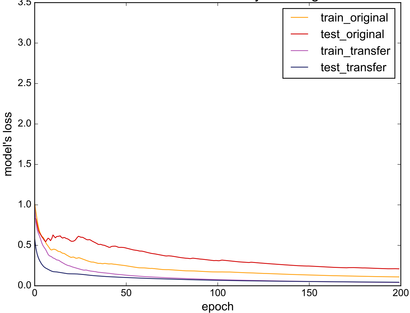
Source: UWaveGestureLibraryAll - Target: CBF
