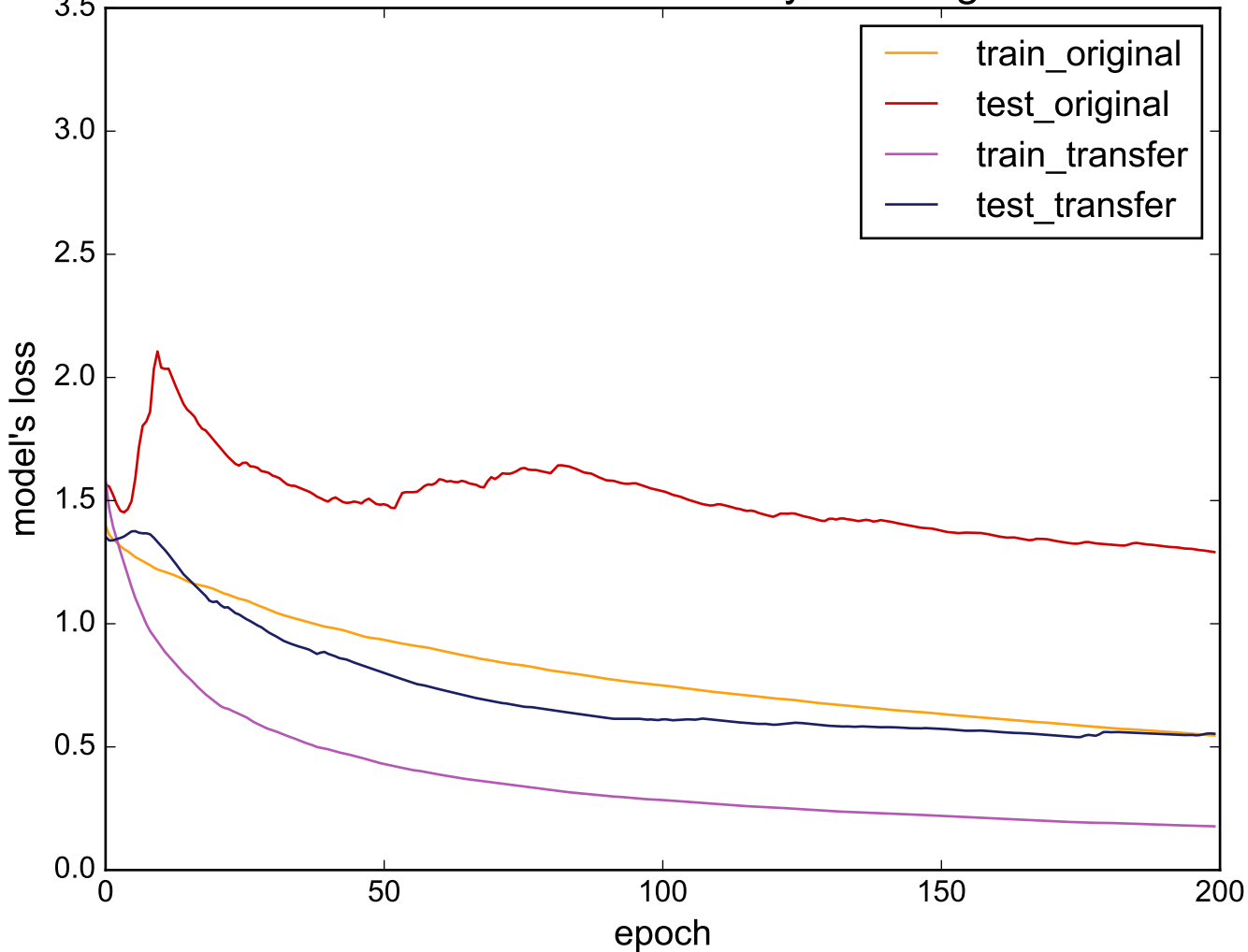
Source: UWaveGestureLibraryAll - Target: Car
