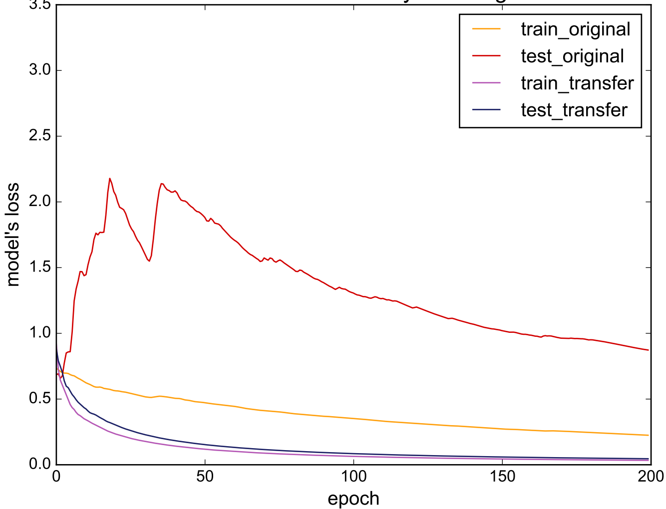
Source: UWaveGestureLibraryAll - Target: Coffee
