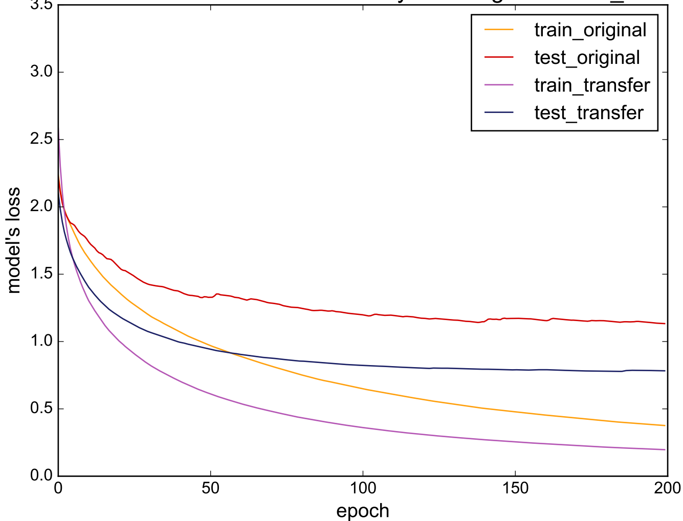
Source: UWaveGestureLibraryAll - Target: Cricket_Y
