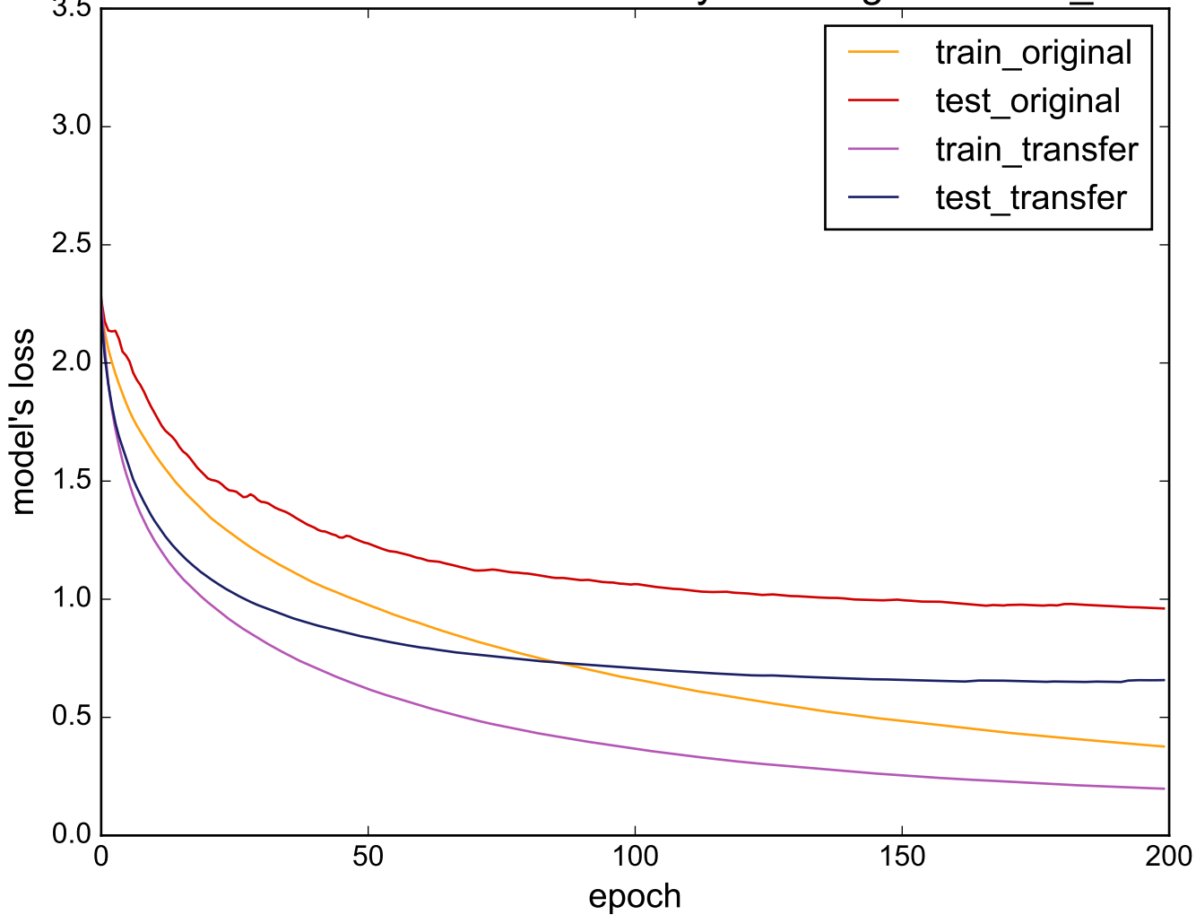
Source: UWaveGestureLibraryAll - Target: Cricket_Z
