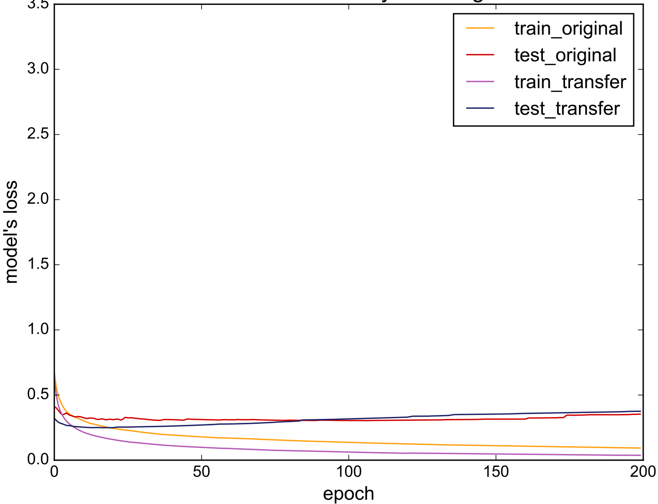
Source: UWaveGestureLibraryAll - Target: ECG5000
