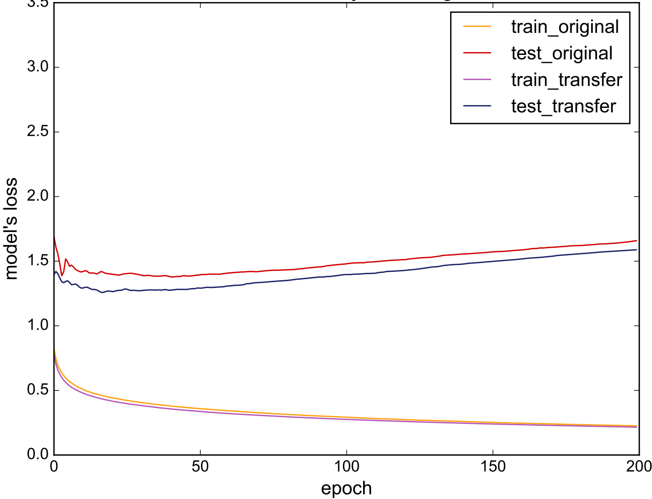
Source: UWaveGestureLibraryAll - Target: ElectricDevices
