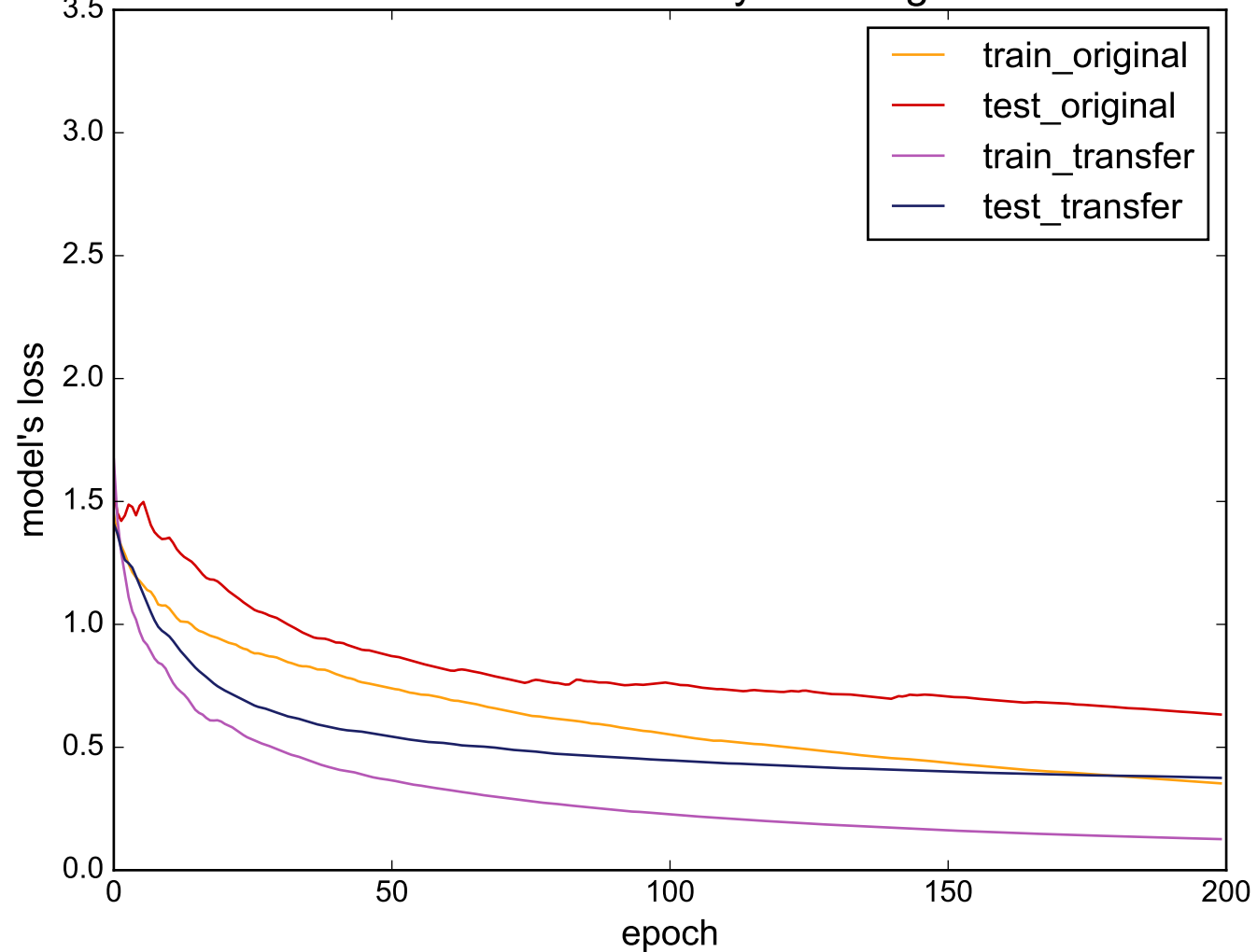
Source: UWaveGestureLibraryAll - Target: FaceFour
