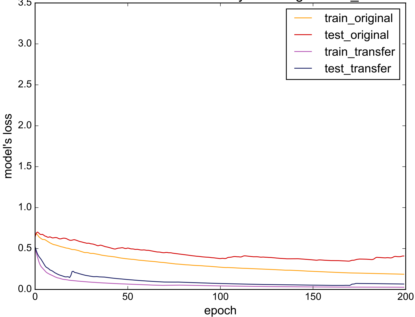
Source: UWaveGestureLibraryAll - Target: Gun_Point
