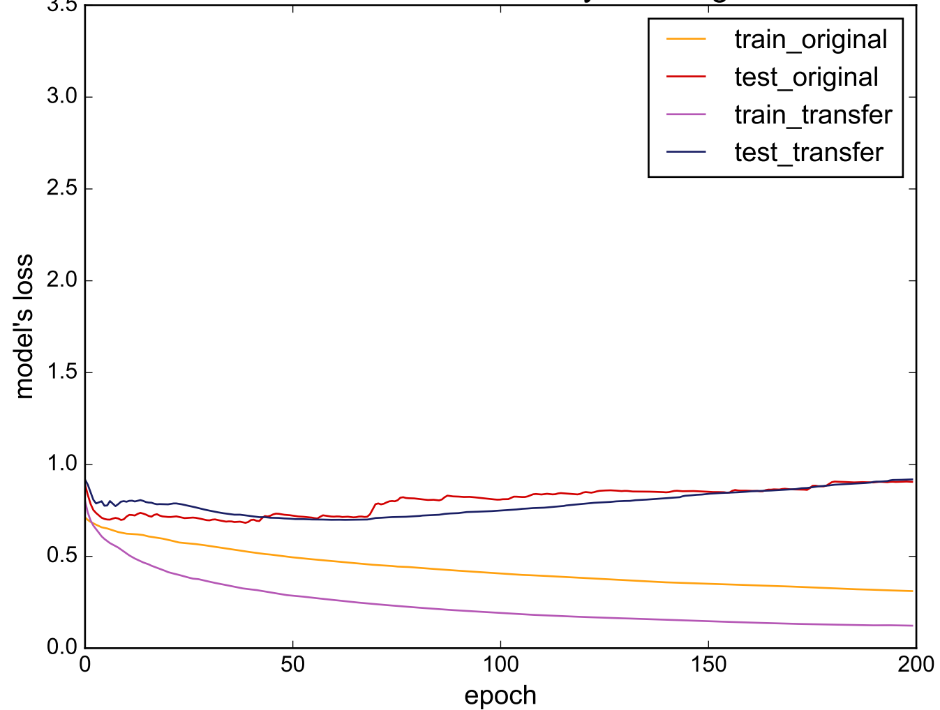
Source: UWaveGestureLibraryAll - Target: Ham
