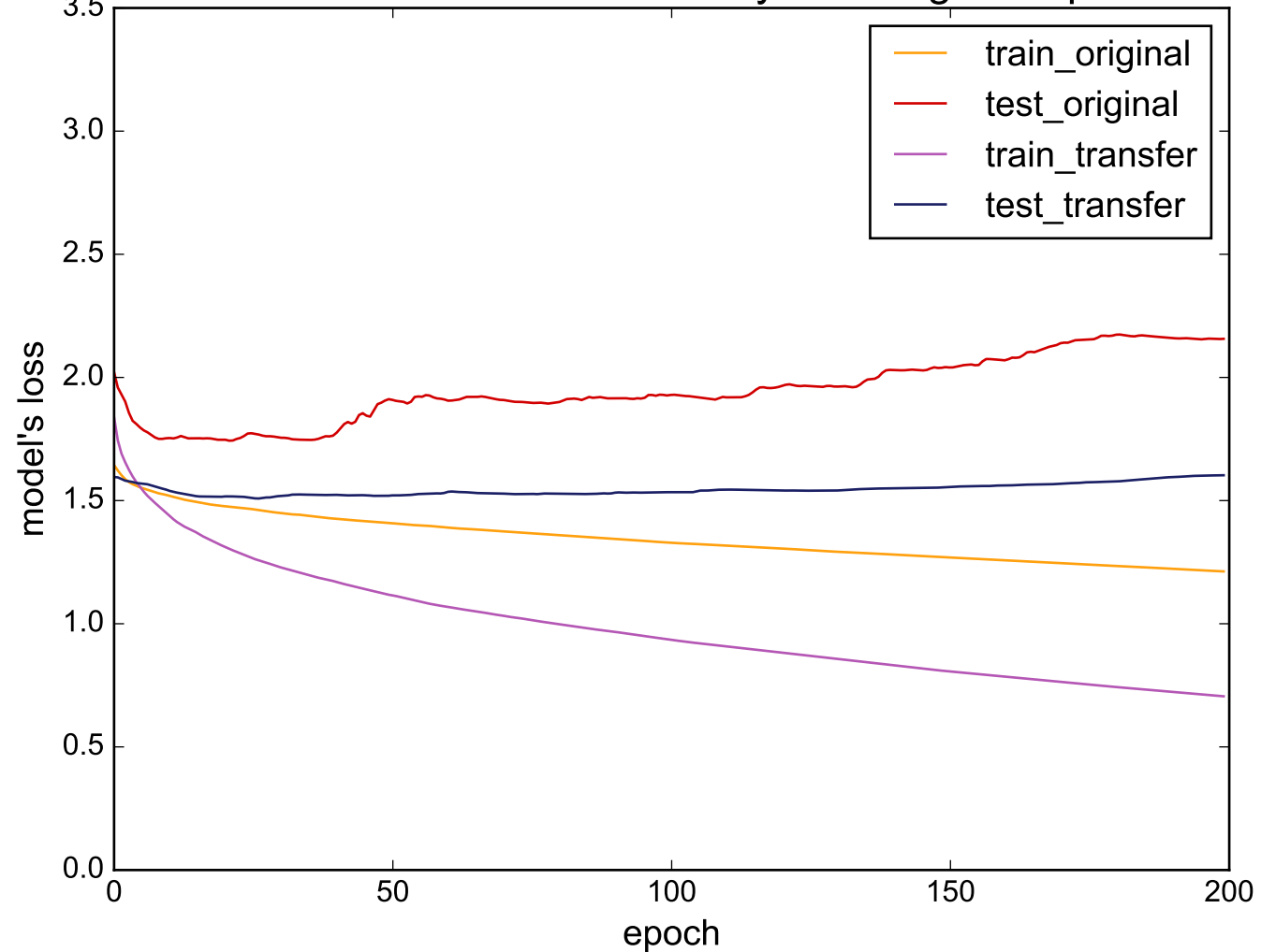
Source: UWaveGestureLibraryAll - Target: Haptics
