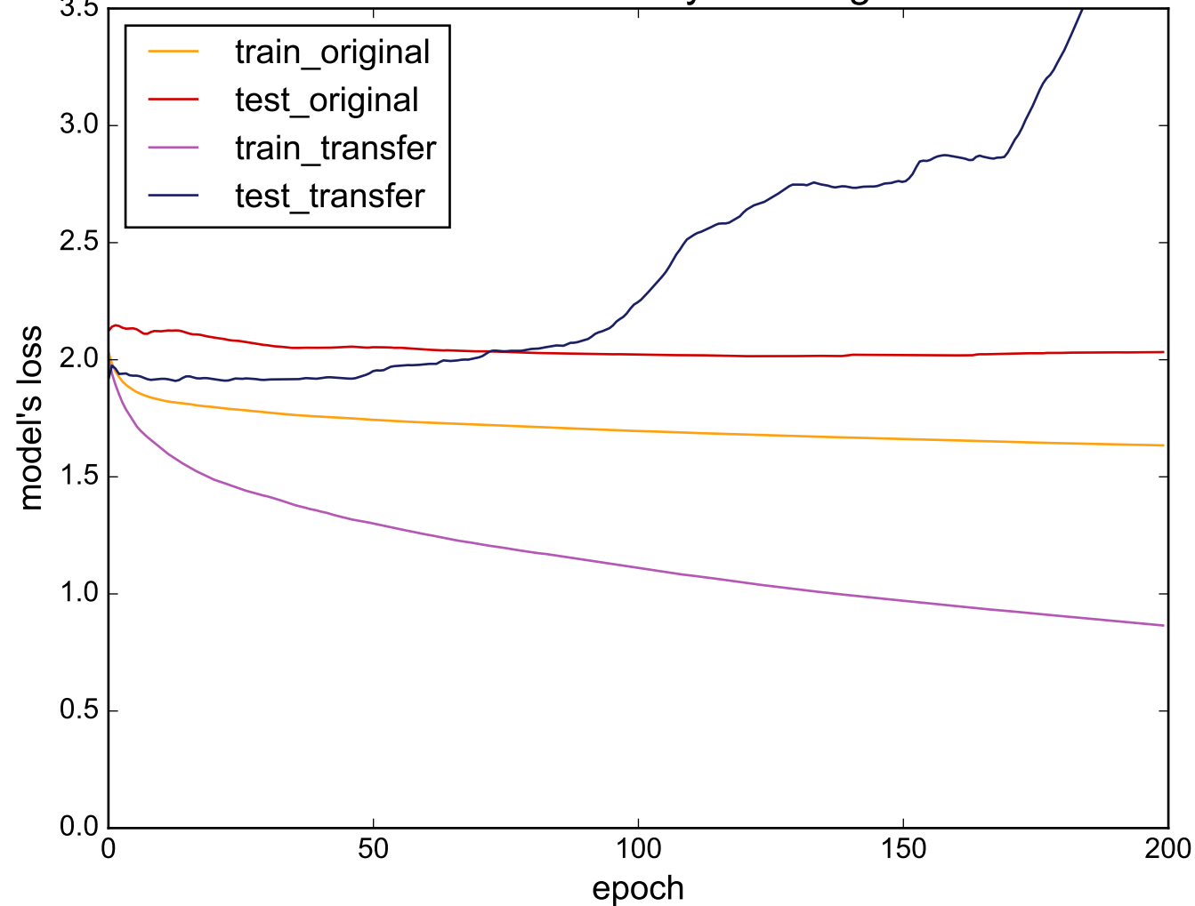
Source: UWaveGestureLibraryAll - Target: InlineSkate
