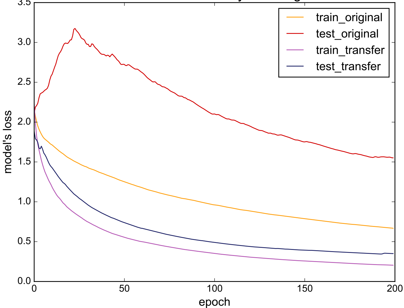
Source: UWaveGestureLibraryAll - Target: MALLAT
