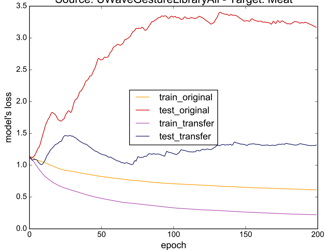
Source: UWaveGestureLibraryAll - Target: Meat
