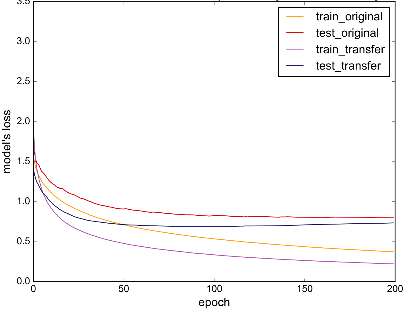
Source: UWaveGestureLibraryAll - Target: MedicalImages
