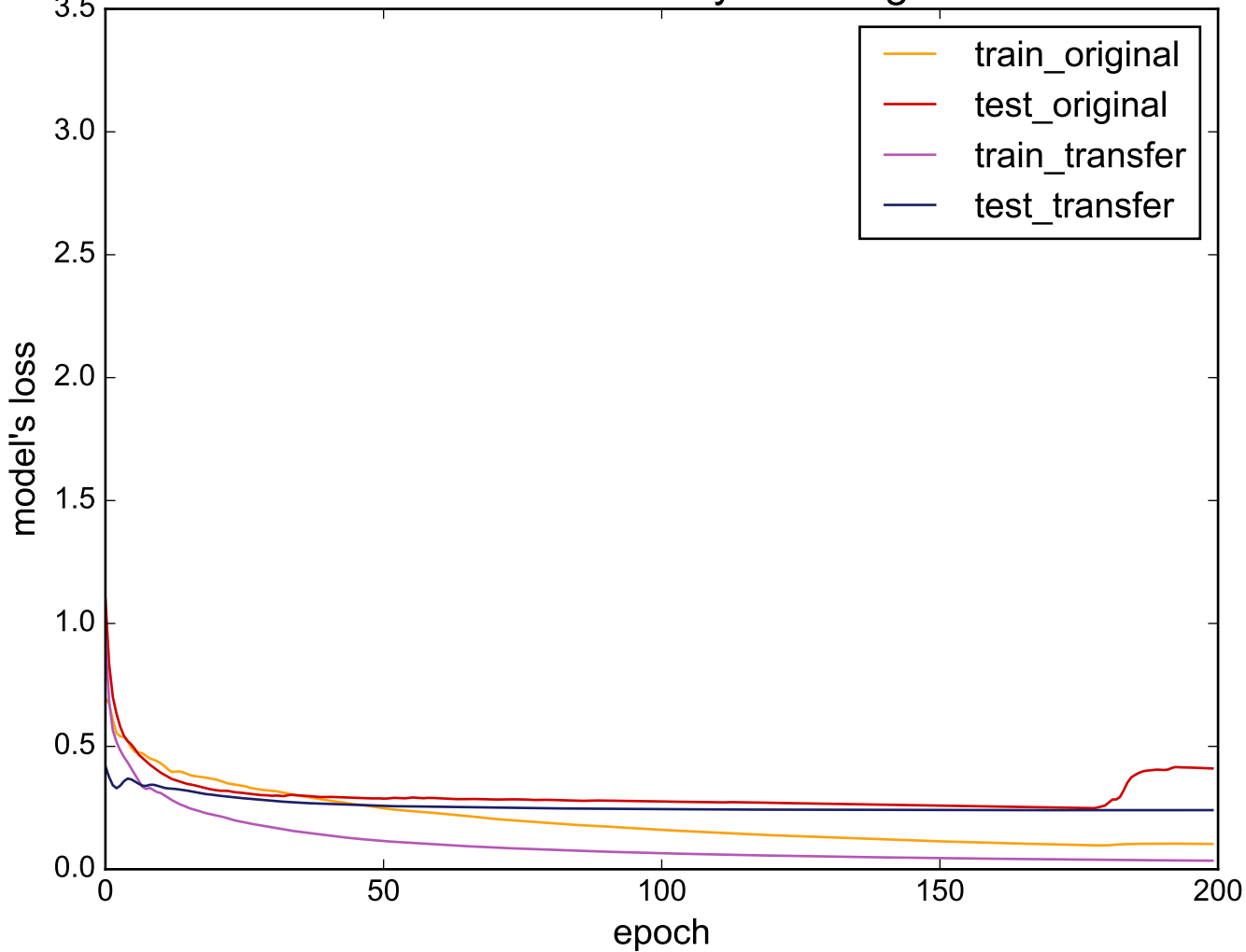
Source: UWaveGestureLibraryAll - Target: MoteStrain
