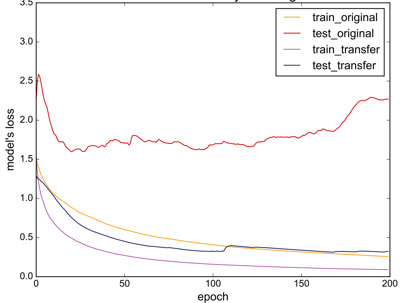
Source: UWaveGestureLibraryAll - Target: OSULeaf
