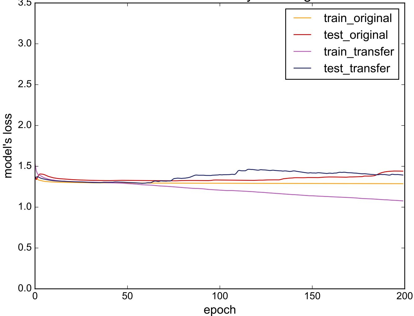
Source: UWaveGestureLibraryAll - Target: OliveOil
