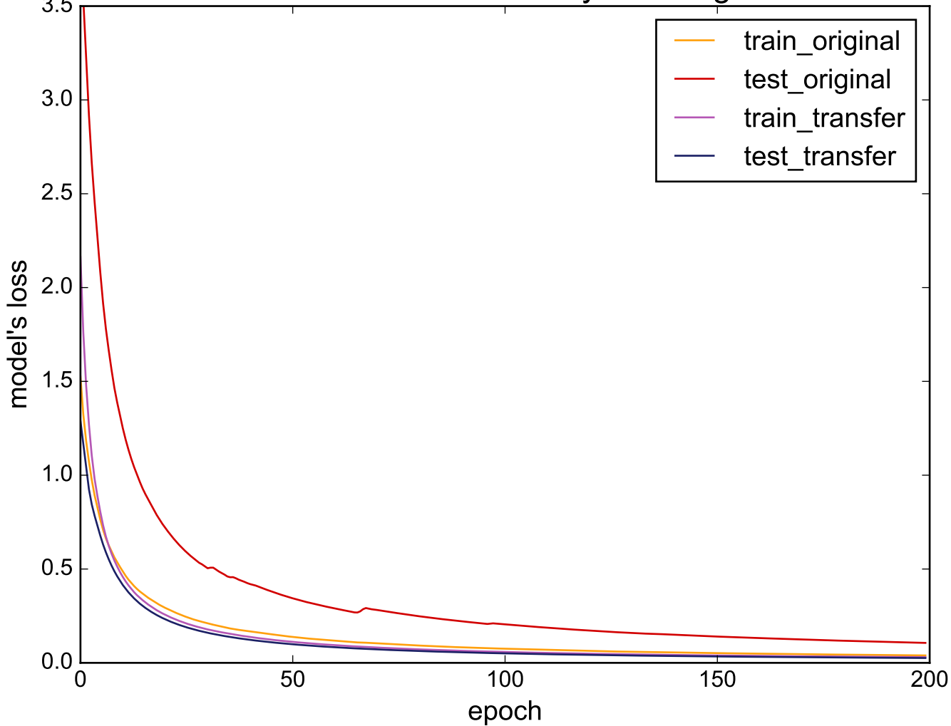
Source: UWaveGestureLibraryAll - Target: Plane
