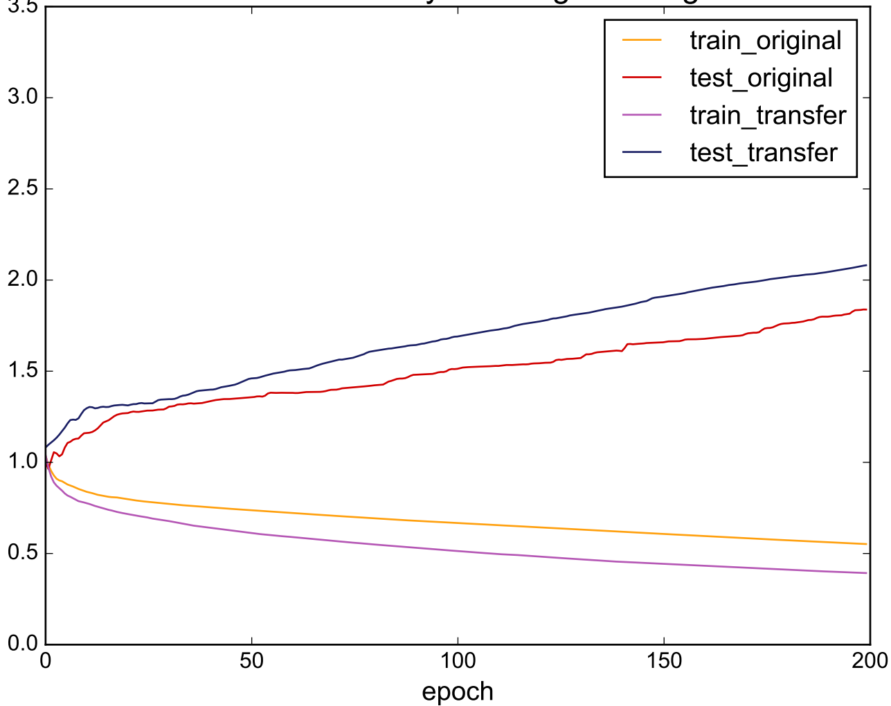
Source: UWaveGestureLibraryAll - Target: RefrigerationDevices
