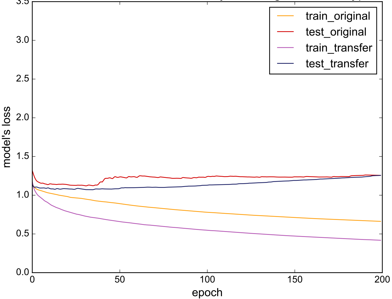
Source: UWaveGestureLibraryAll - Target: ScreenType
