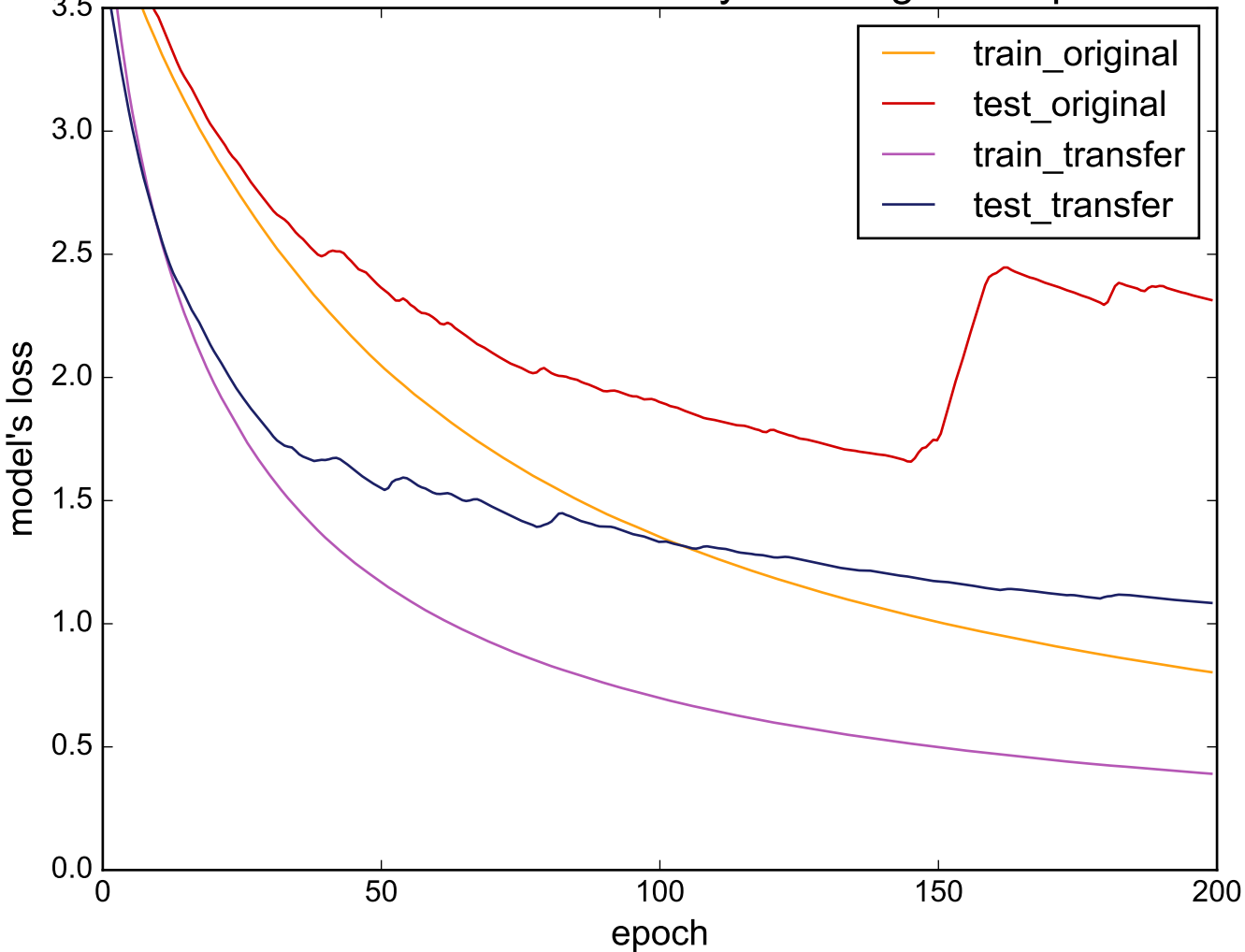
Source: UWaveGestureLibraryAll - Target: ShapesAll
