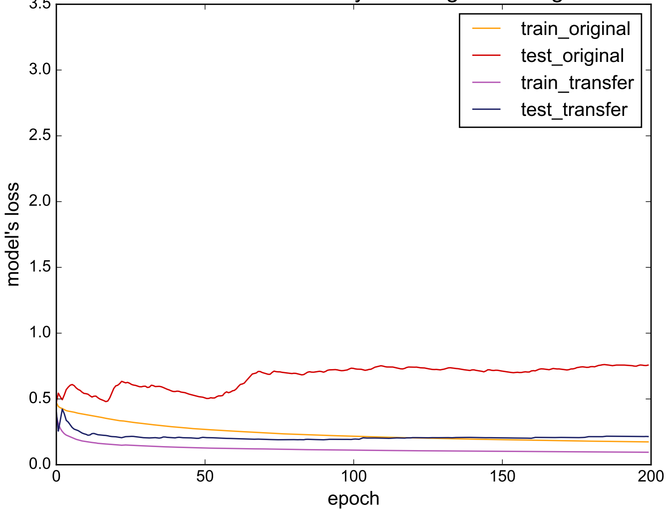
Source: UWaveGestureLibraryAll - Target: StarLightCurves
