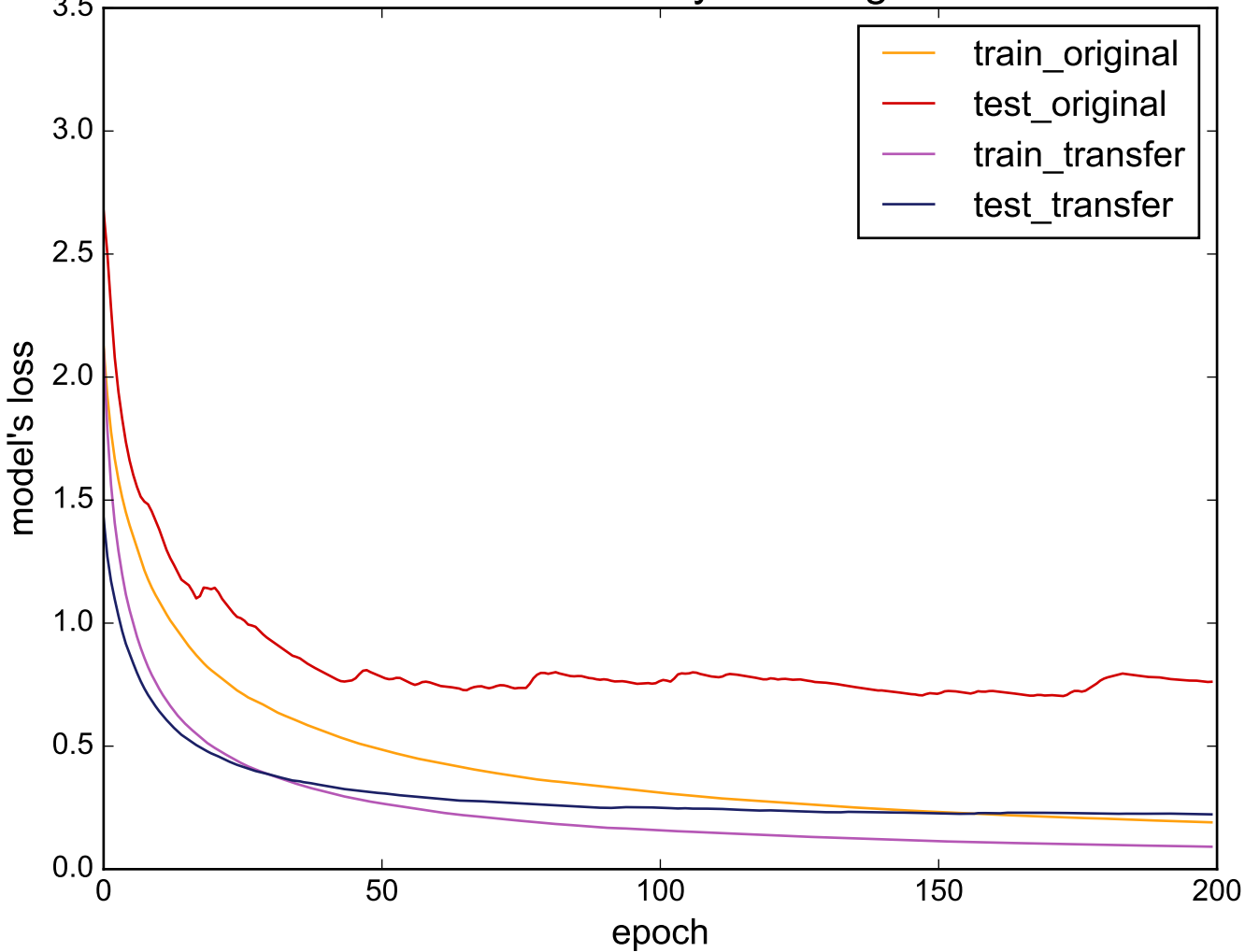
Source: UWaveGestureLibraryAll - Target: SwedishLeaf
