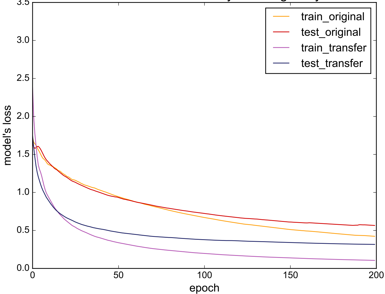
Source: UWaveGestureLibraryAll - Target: Symbols
