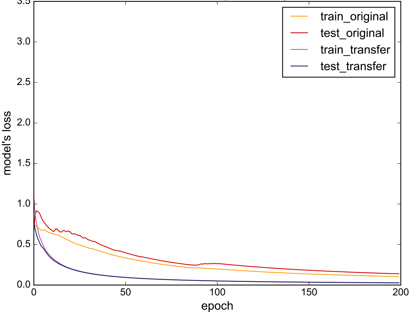
Source: UWaveGestureLibraryAll - Target: TwoLeadECG
