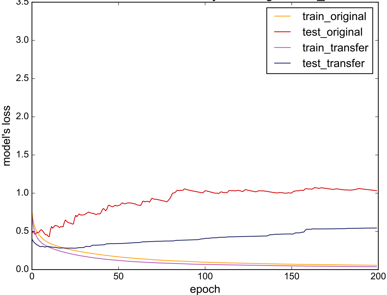
Source: UWaveGestureLibraryAll - Target: Two_Patterns
