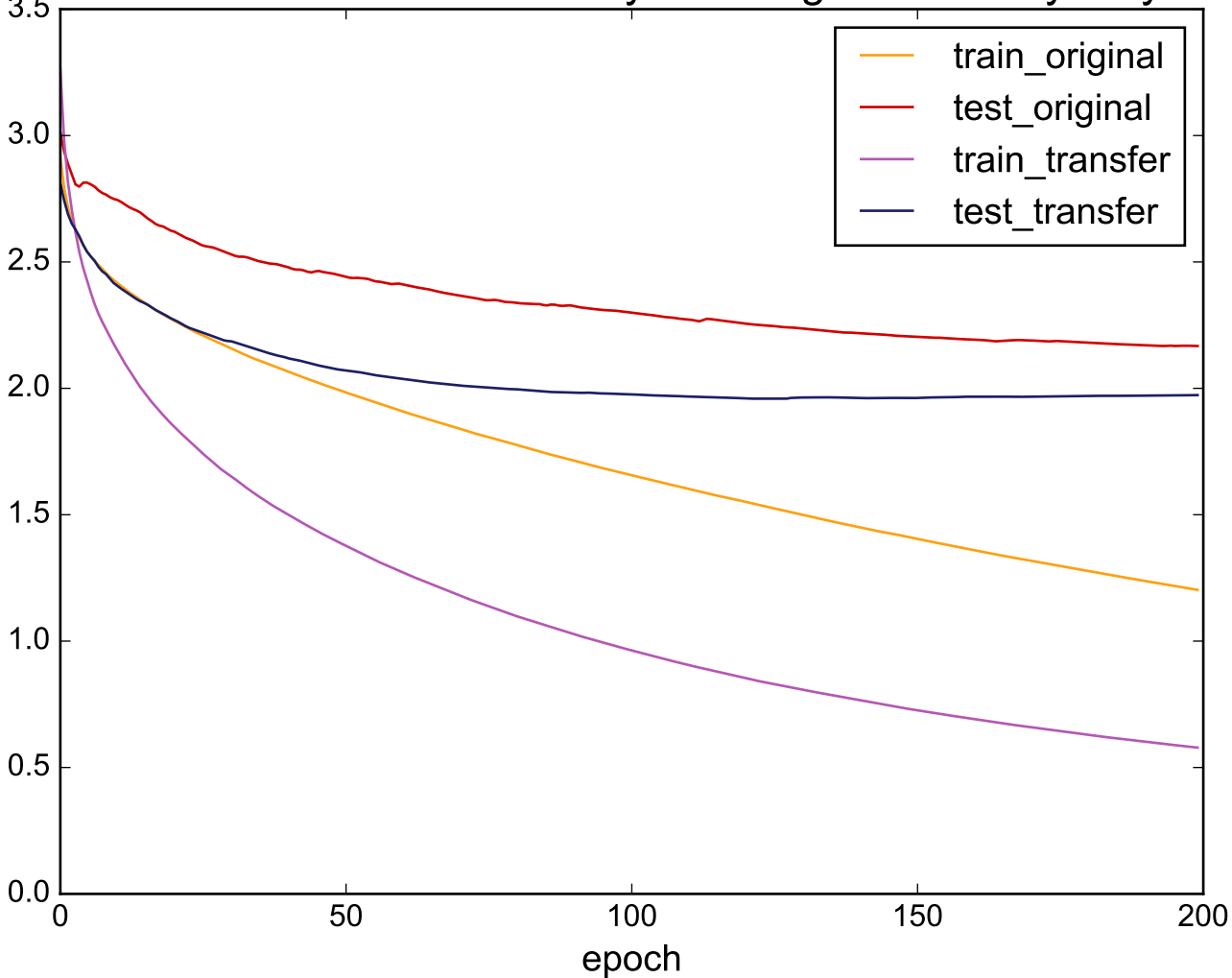
Source: UWaveGestureLibraryAll - Target: WordsSynonyms
