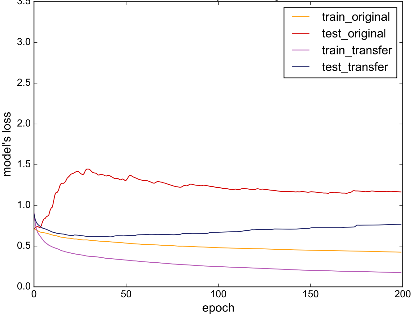
Source: UWaveGestureLibraryAll - Target: WormsTwoClass
