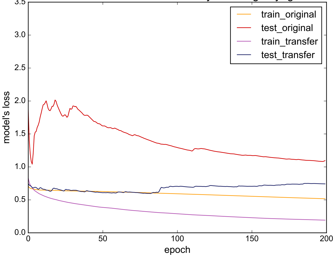
Source: UWaveGestureLibraryAll - Target: yoga
