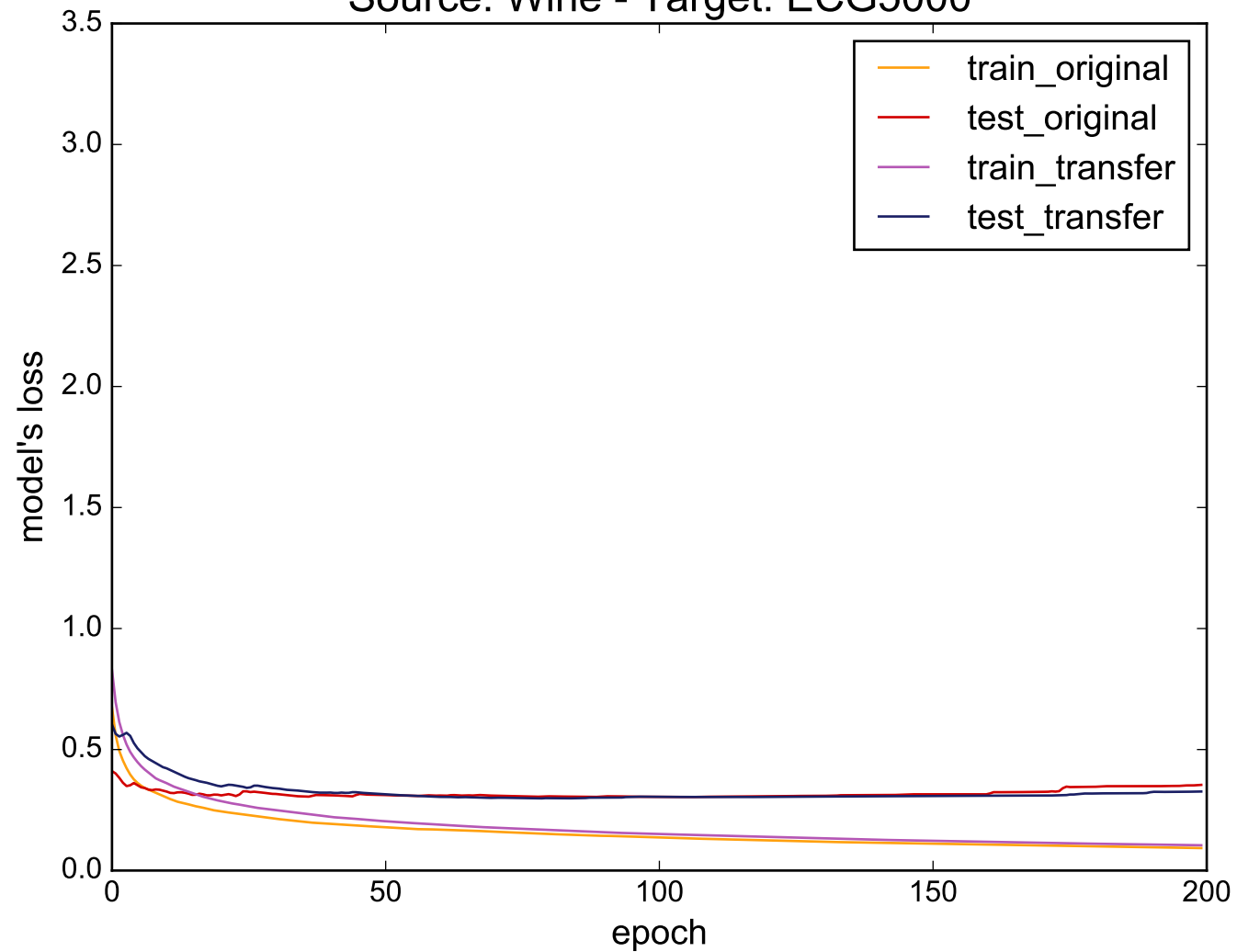
Source: Wine - Target: ECG5000
