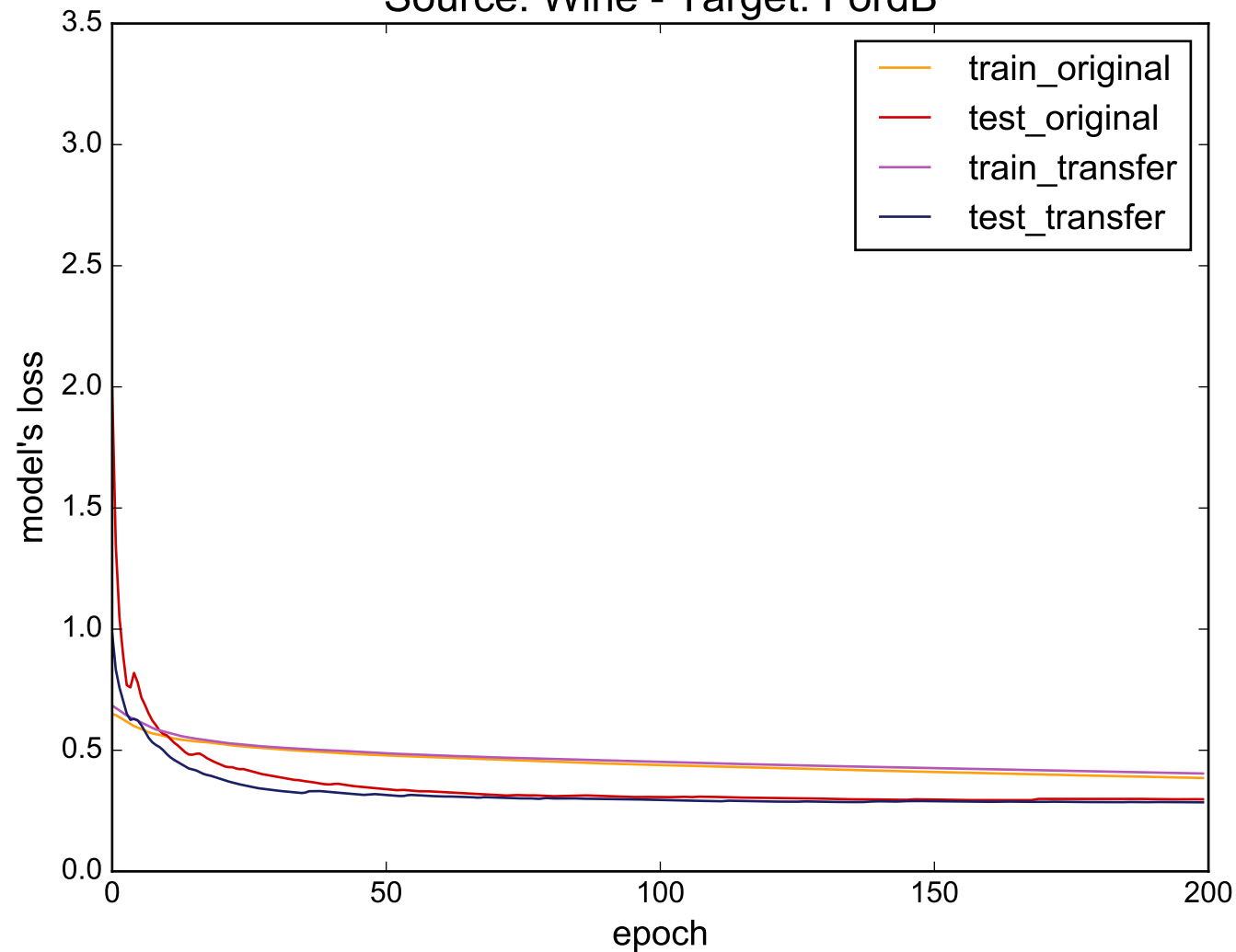
Source: Wine - Target: FordB
