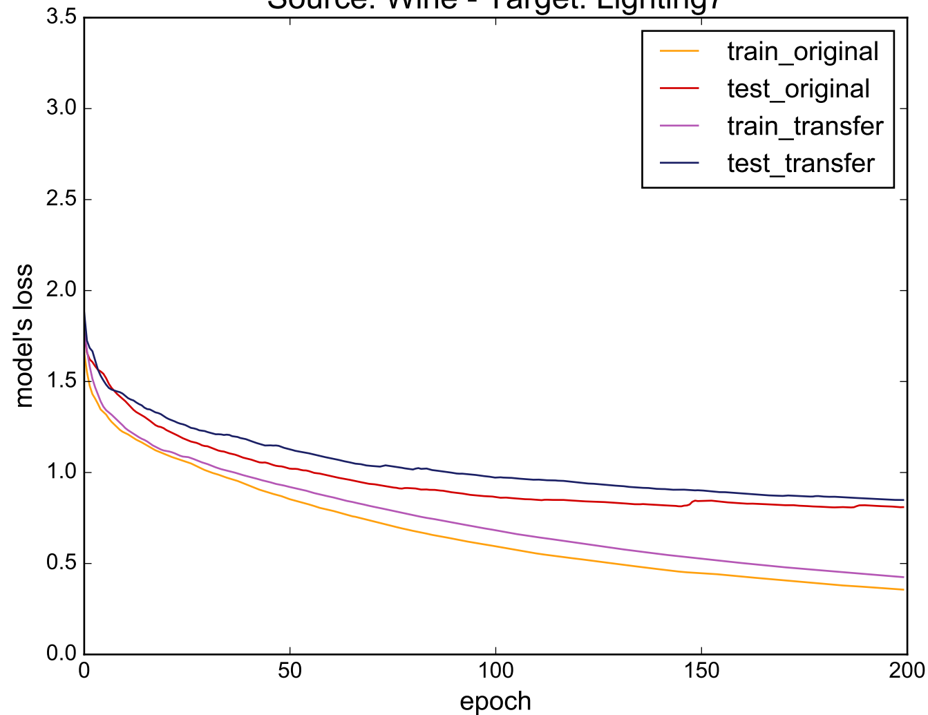
Source: Wine - Target: Lighting7
