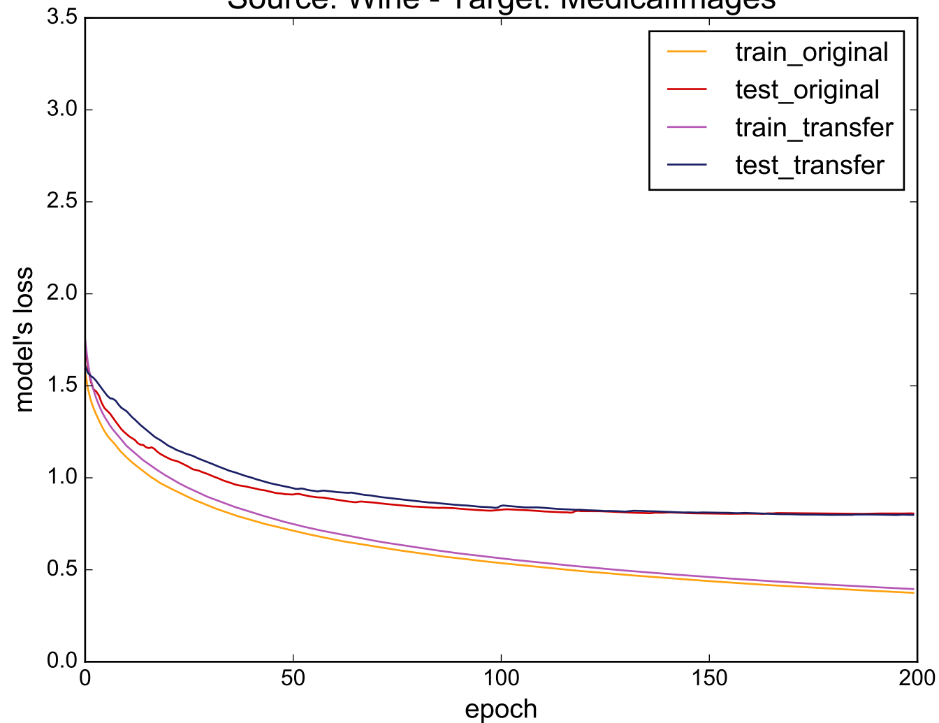
Source: Wine - Target: MedicalImages
