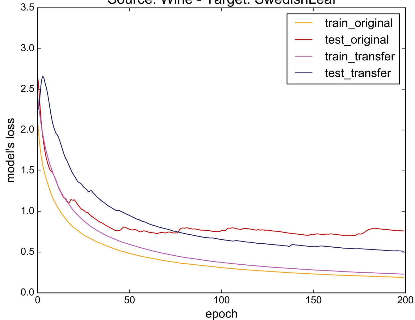
Source: Wine - Target: SwedishLeaf
