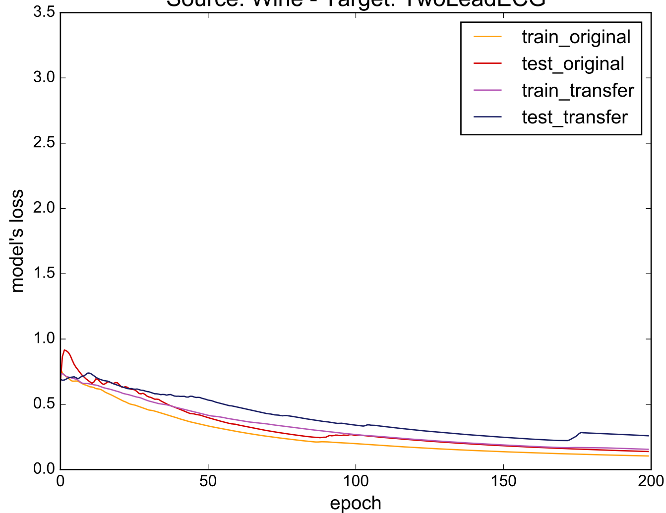
Source: Wine - Target: TwoLeadECG
