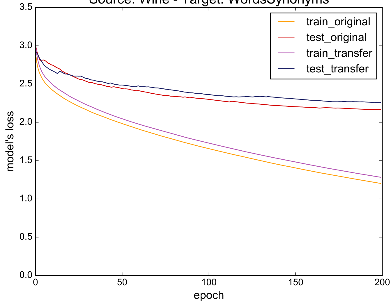
Source: Wine - Target: WordsSynonyms
