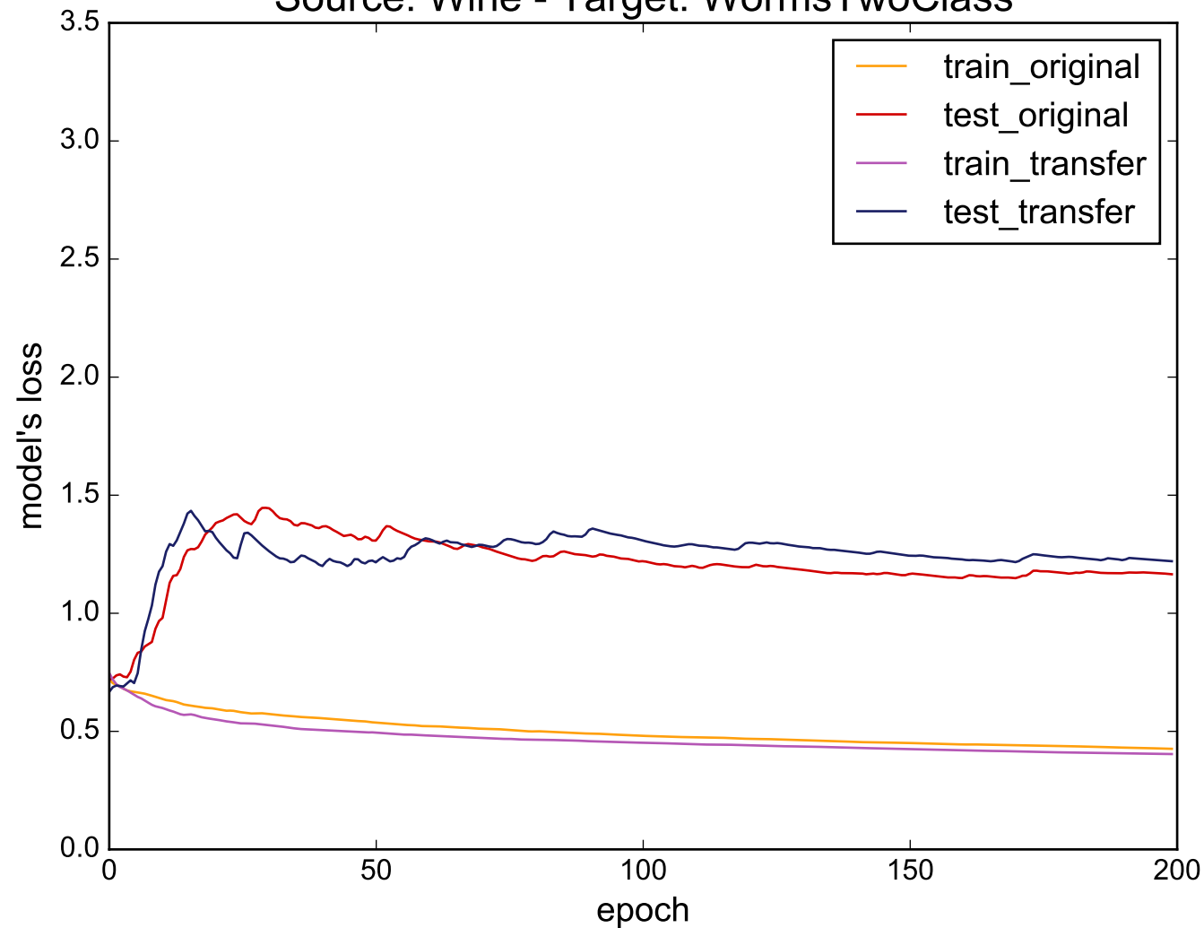
Source: Wine - Target: WormsTwoClass
