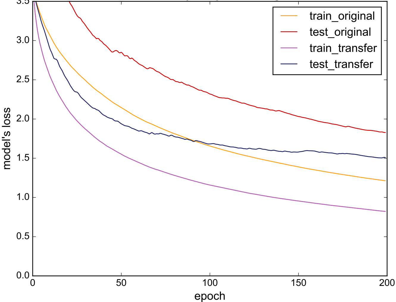
Source: WordsSynonyms - Target: Adiac
