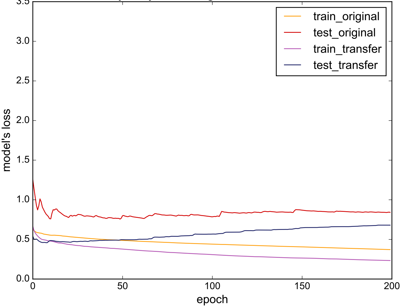
Source: WordsSynonyms - Target: DistalPhalanxOutlineCorrect
