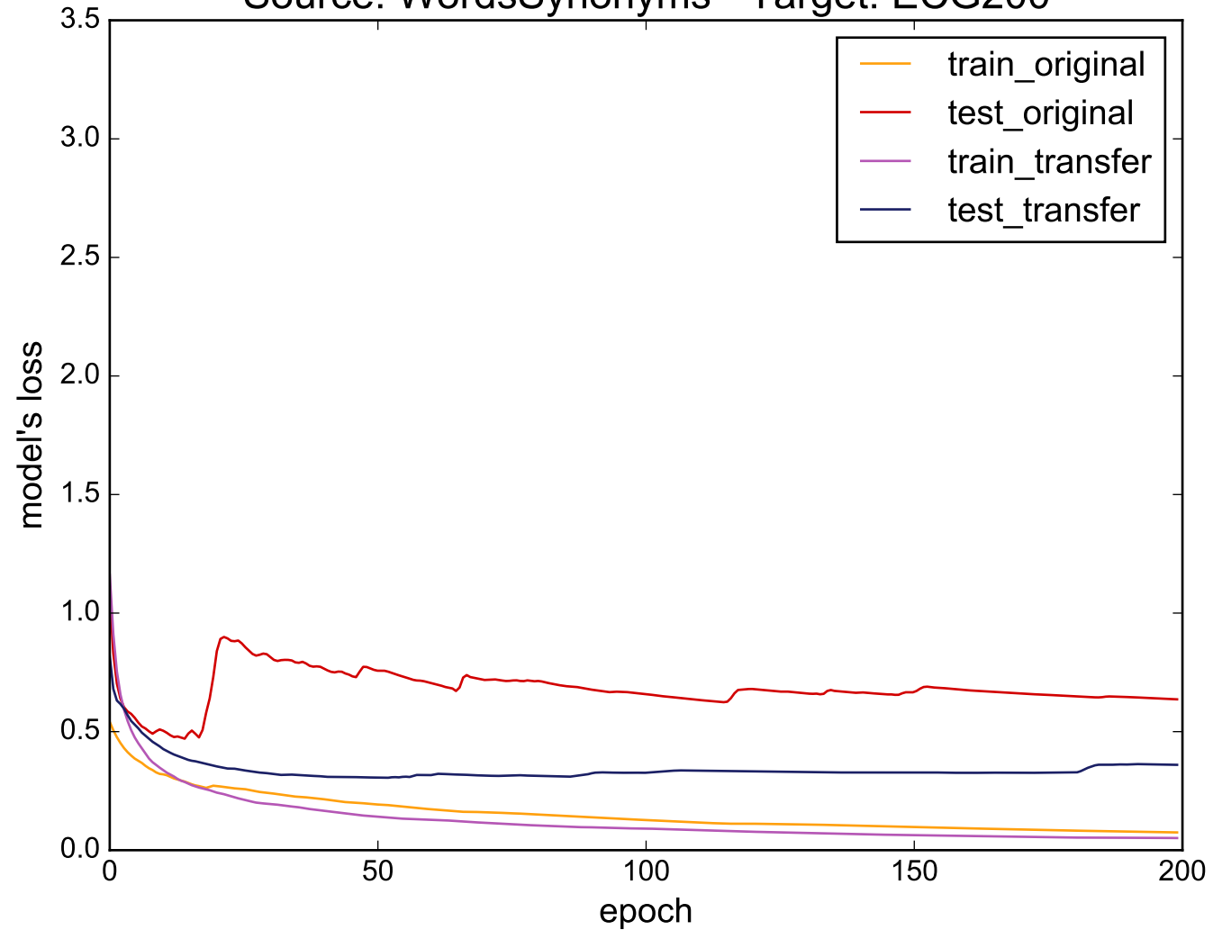
Source: WordsSynonyms - Target: ECG200
