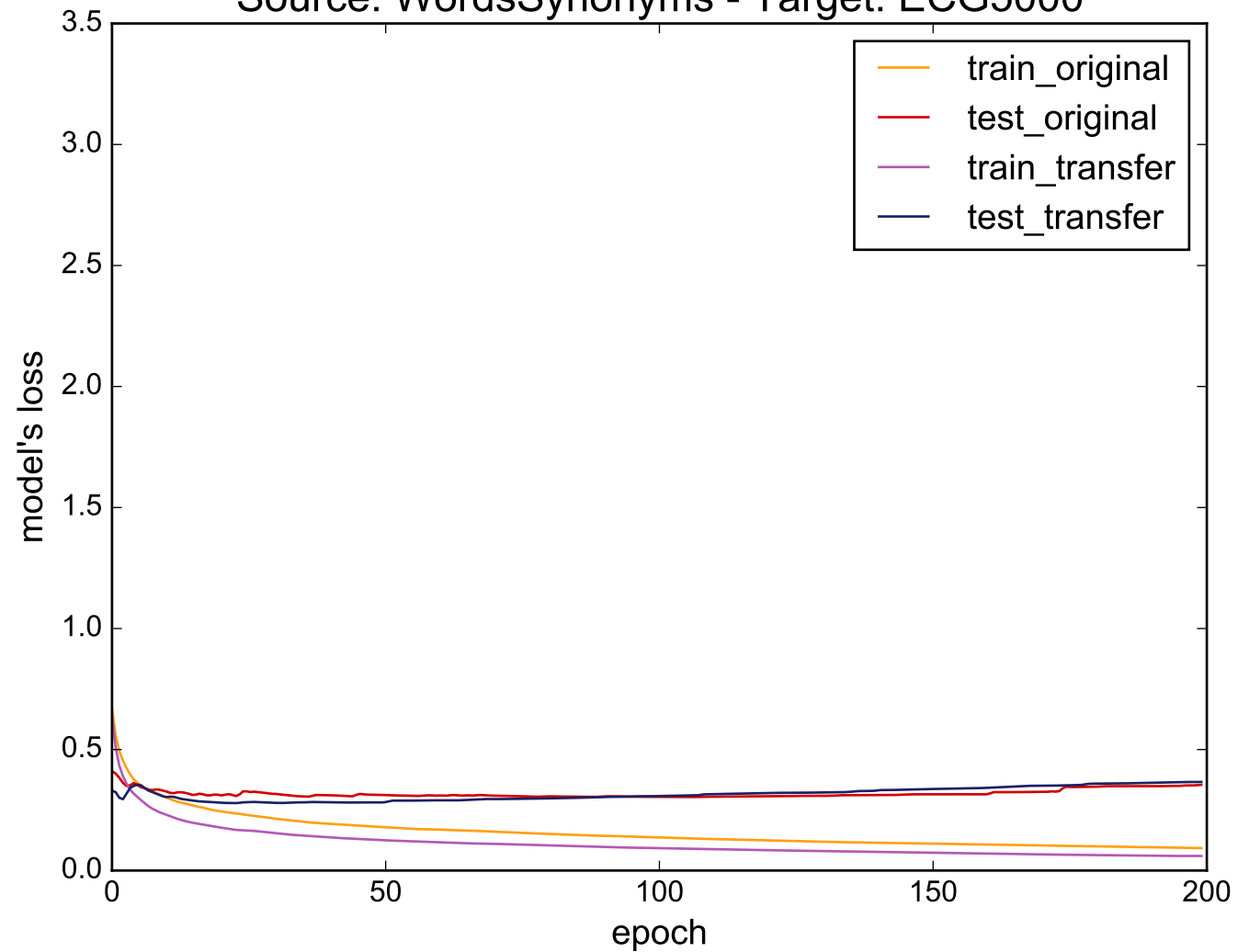
Source: WordsSynonyms - Target: ECG5000
