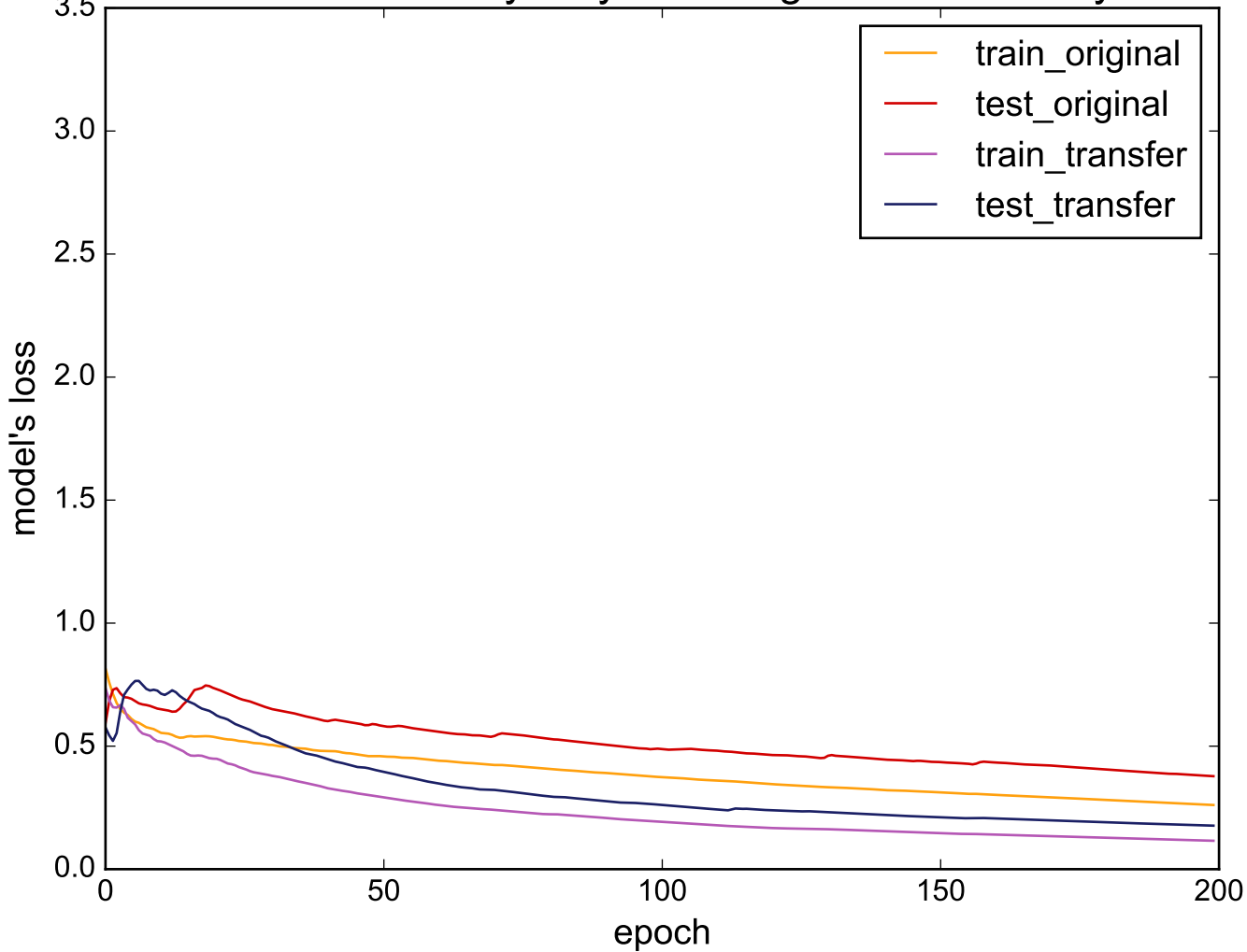
Source: WordsSynonyms - Target: ECGFiveDays
